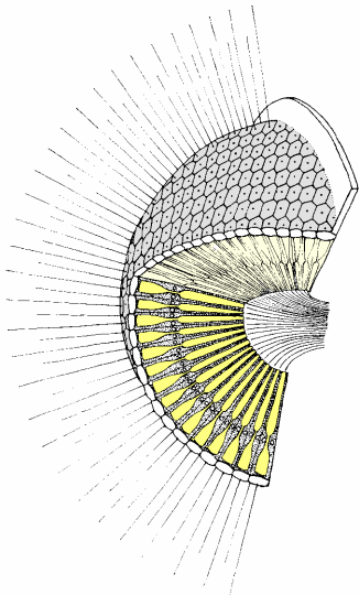
Facettenauge
